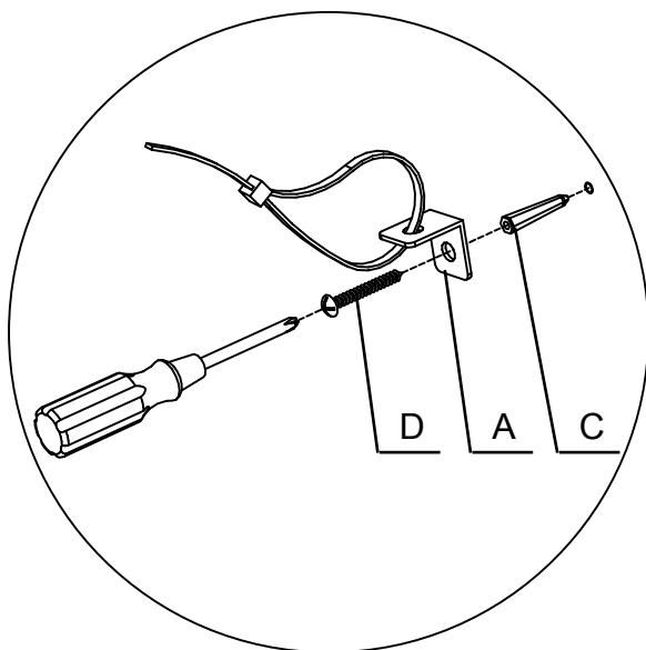
Masonry wall mounting
