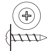
H10 x 1 TRUSS-HEAD SCREW
